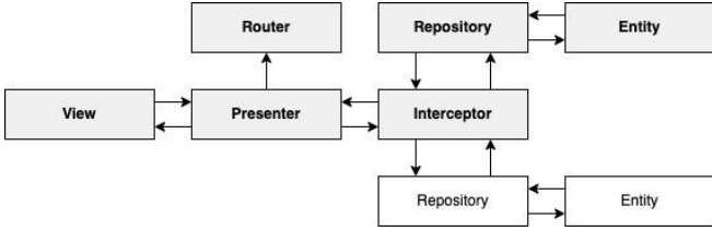
Fig 4. VIPER architecture
