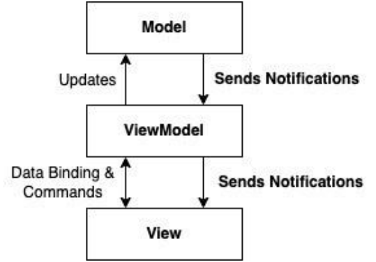
Fig. 2 MVVM architecture
